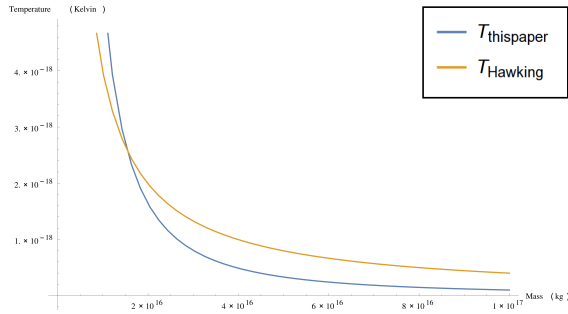
Figure 2: Black Hole Temperature as a Function of Mass. Here is a plot of the famous result due to Stephen Hawking along with a result from my own model published in 2014 Farmer [2015a,b]. In this model black holes produce Hawking radiation at a rate which is compatible with observations yet differs from Hawkings prediction. To see which is correct would take so long as to be impractical. So I will propose a simple experiment in this paper. (“This paper” refers to Farmer [2015a].)
